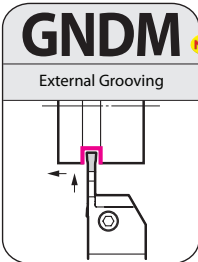
Use for multi-purpose or profiling insert for turning (widening).
